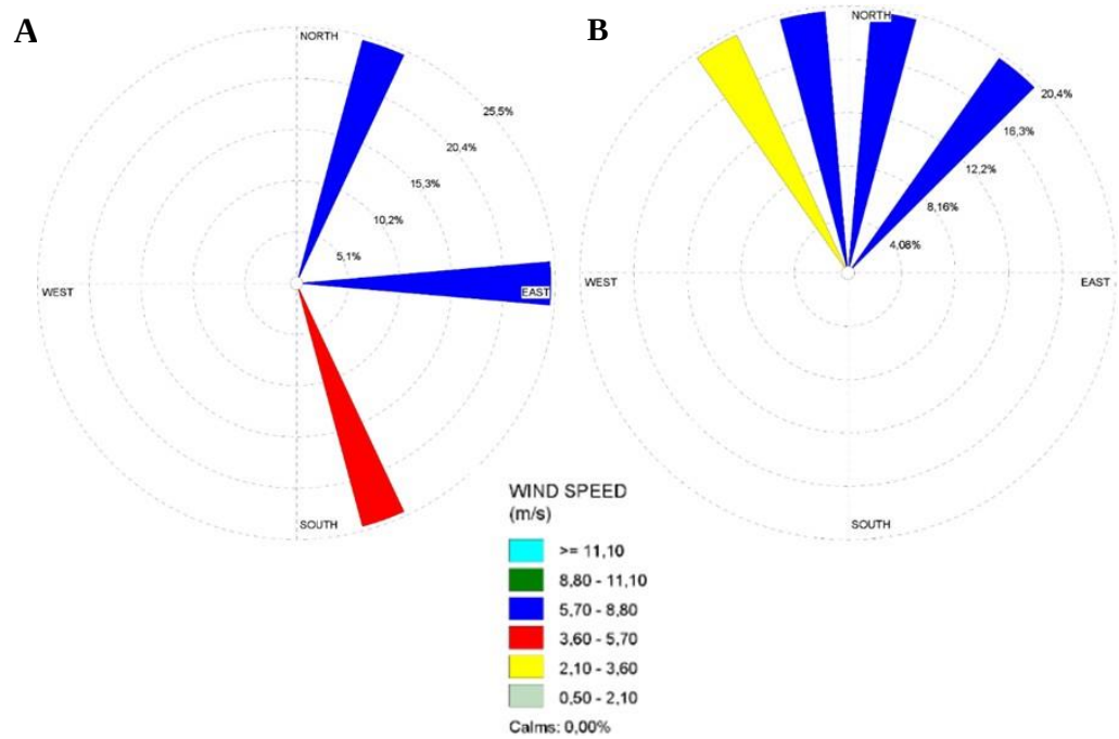
Figure S1. Wind conditions recorded during microplastics collections in surface waters in the Santos Basin.
