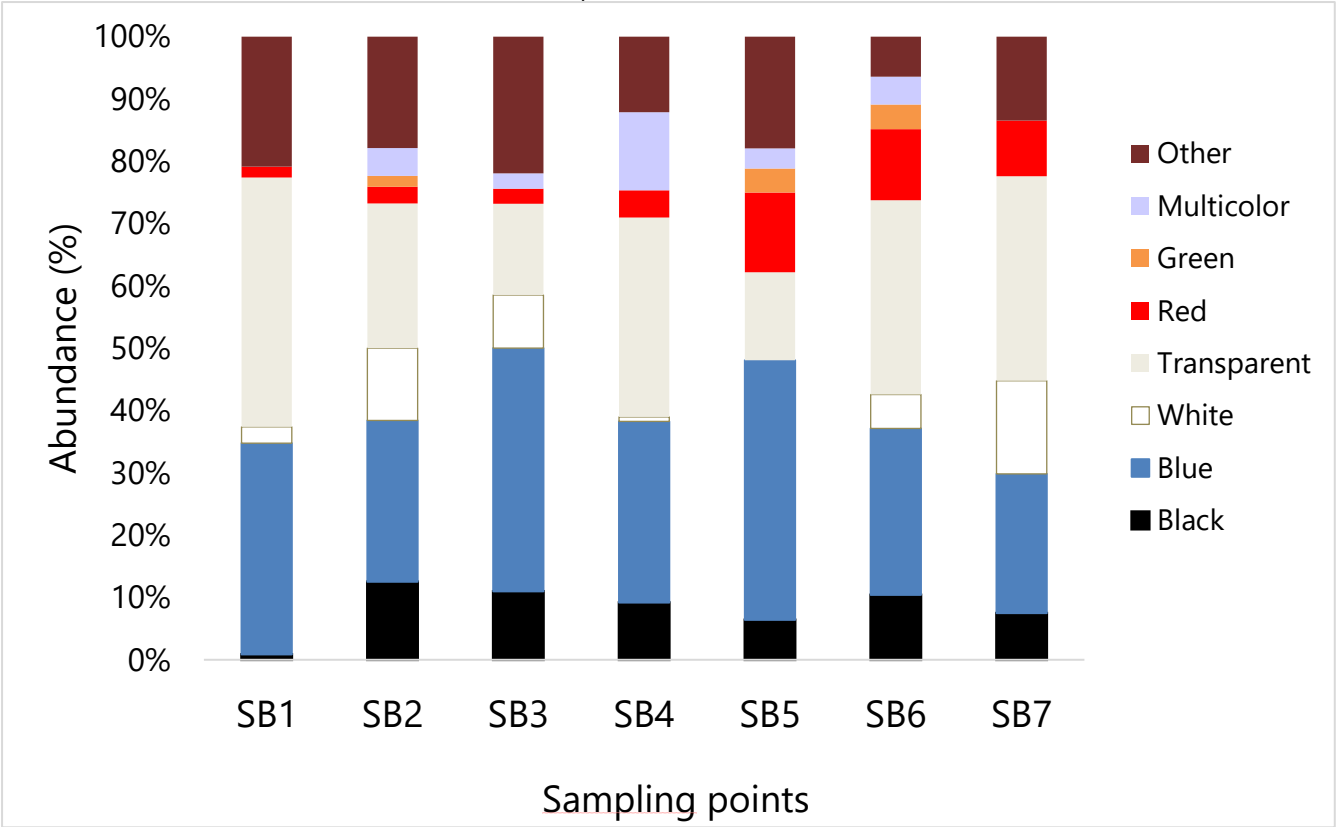
Caption: SB, Santos Basin.
