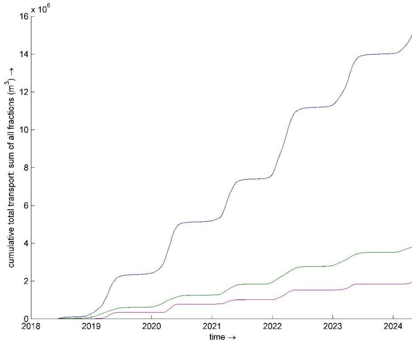
Figure SP 4. Total cumulative transport for the upstream section of the Pimental reservoir for the period between 06/11/2018 and 05/09/2024. In blue: Upstream; Green: Diversion Channel; Purple: Spillway.
