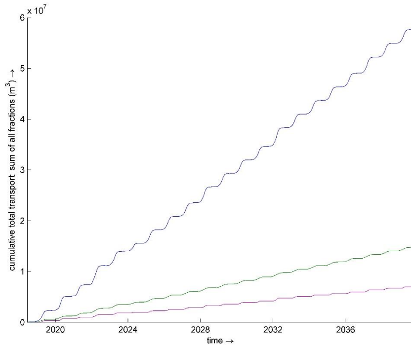
Figure SP 5. Total cumulative transport for the upstream section of the Pimental reservoir for the period between 06/11/2018 and 30/09/2039. In blue: Upstream; Green: Diversion Channel; Purple: Spillway.
