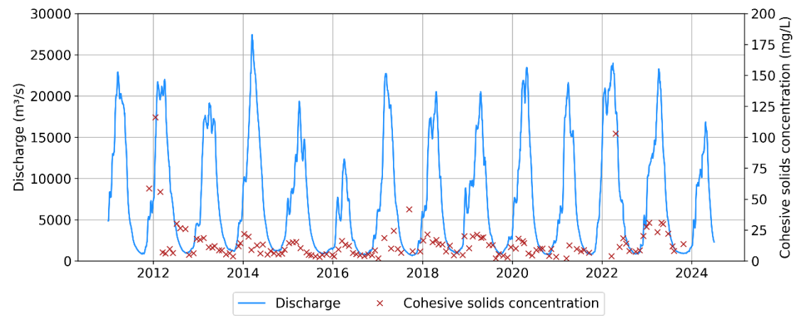
Figure SP 1. Temporal arrangement of suspended solids concentration measurements in relation to liquid flow rate
