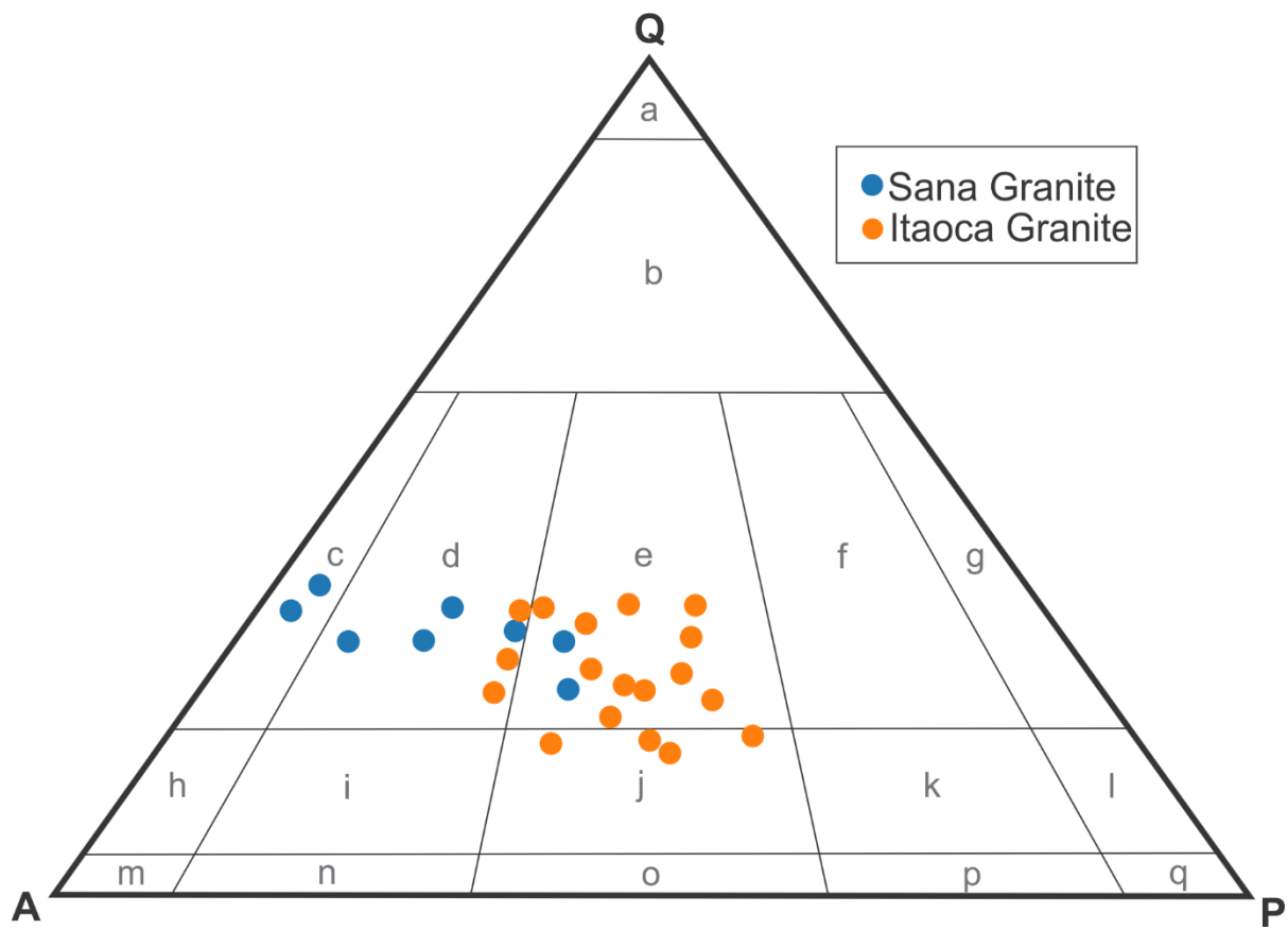
Figure S2: QAP diagram with Sana and Itaoca granite samples.
