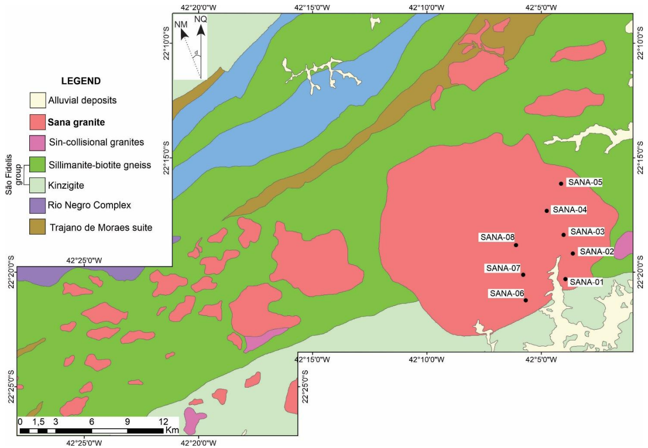
Figure S1: Geological map of the Sana Granite with the positioning of the sample collection points.
