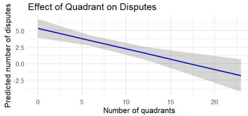
Figure S2. Linear regressions depicting the effect of the mean number of adult females, adult males, and quadrants on dispute frequency.
