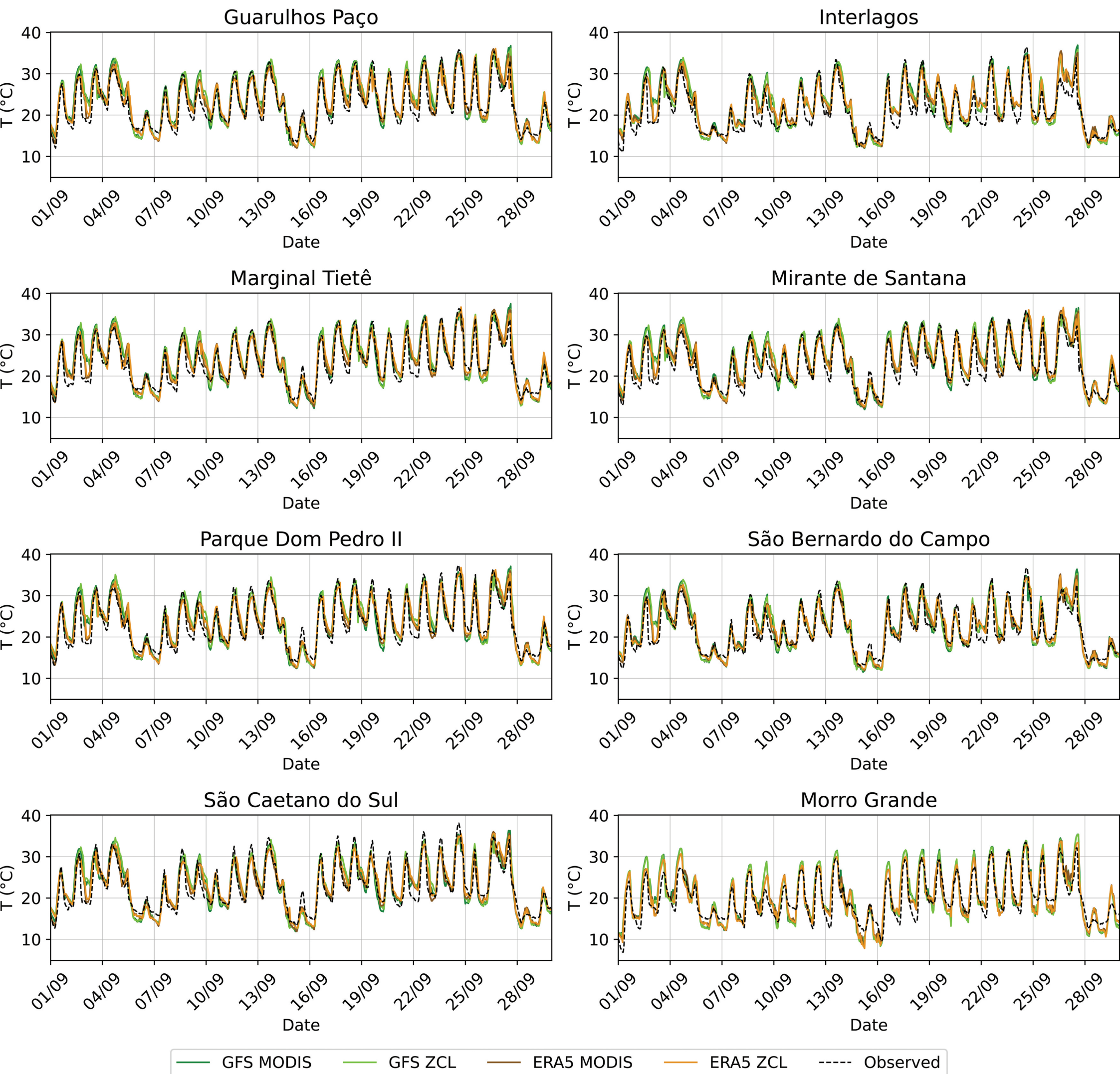
Figure S1. Observed and simulated data in the four experiments for 2-meter air temperature in September 2023.
