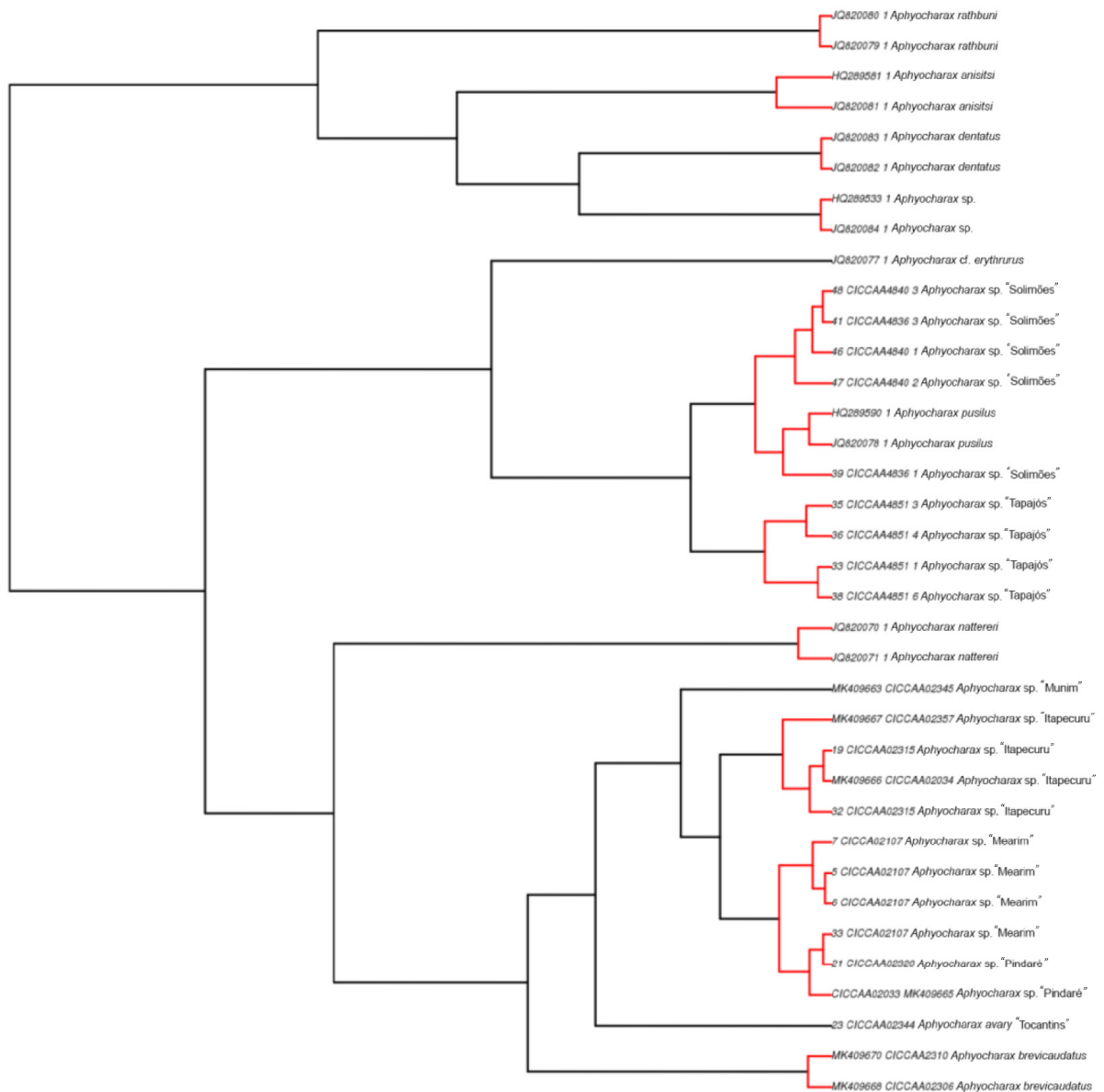
FIGURE S1 | GMYC test analysis. We found the same result to the ingroup, when compared to the result presented in Fig. 3.
