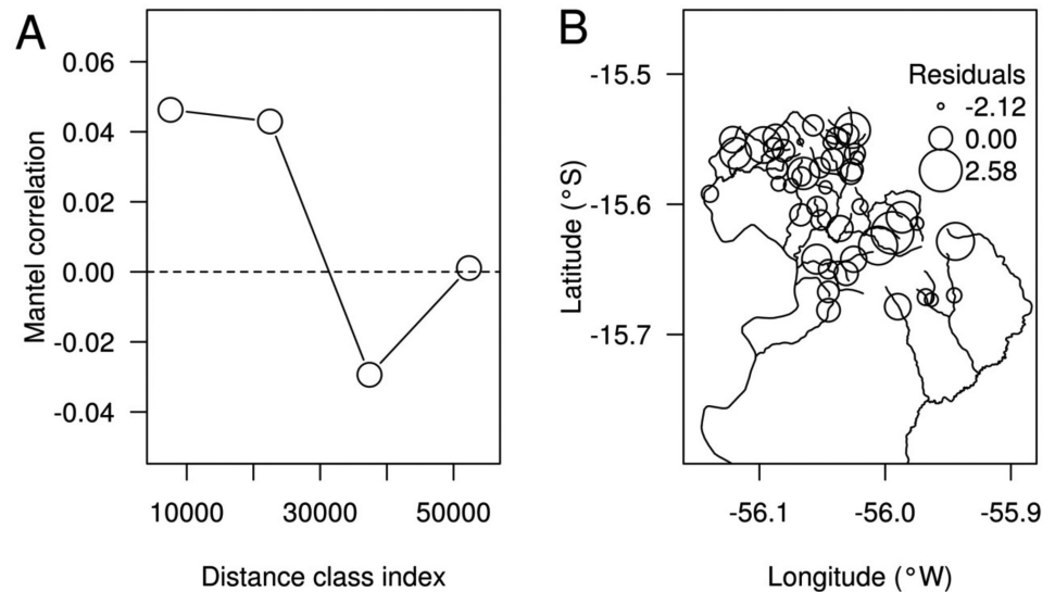
FIGURE S6 | Assessment of spatial autocorrelation in residual distribution of linear model with rarefied species richness as the response variable. Spatial autocorrelation assessed with Mantel correlogram (A) and bubble plot (B).
