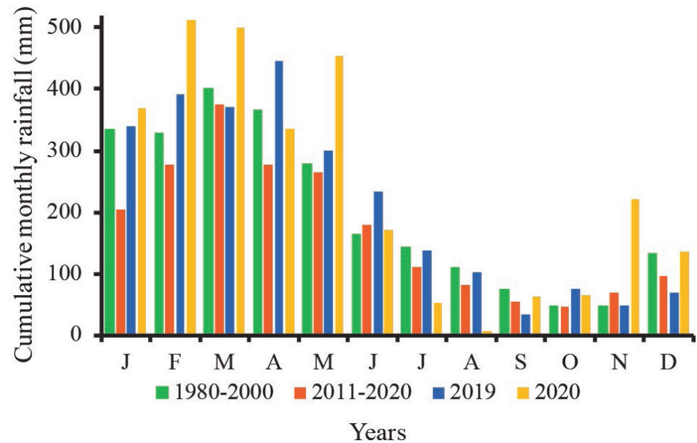
FIGURE S1 | Historical monthly average rainfall records in the municipality of Capitão Poço between 1980 to 2000 (Pacheco, Bastos, 2001), between 2011 to 2020 (INMET, 2021), and separately for 2019 and 2020.
