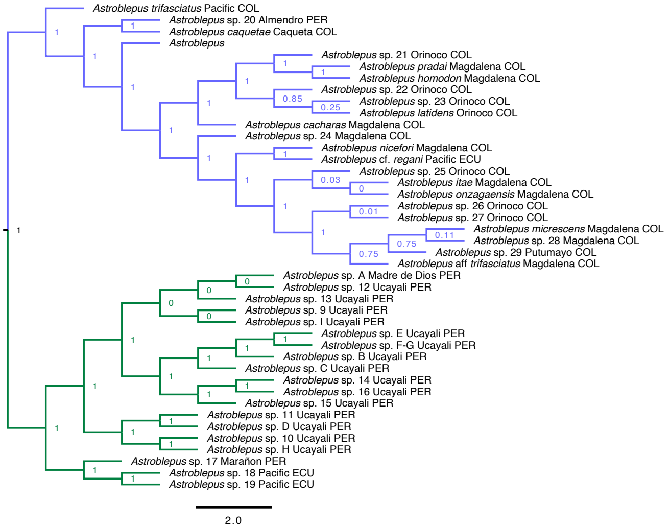
SUPPLEMENTARY MATERIAL FIGURE S4 | Results from BP&P-A10 analysis using gamma-distributed priors for ancestral \theta with a default prior \theta \sim G(3, 0.004) .
