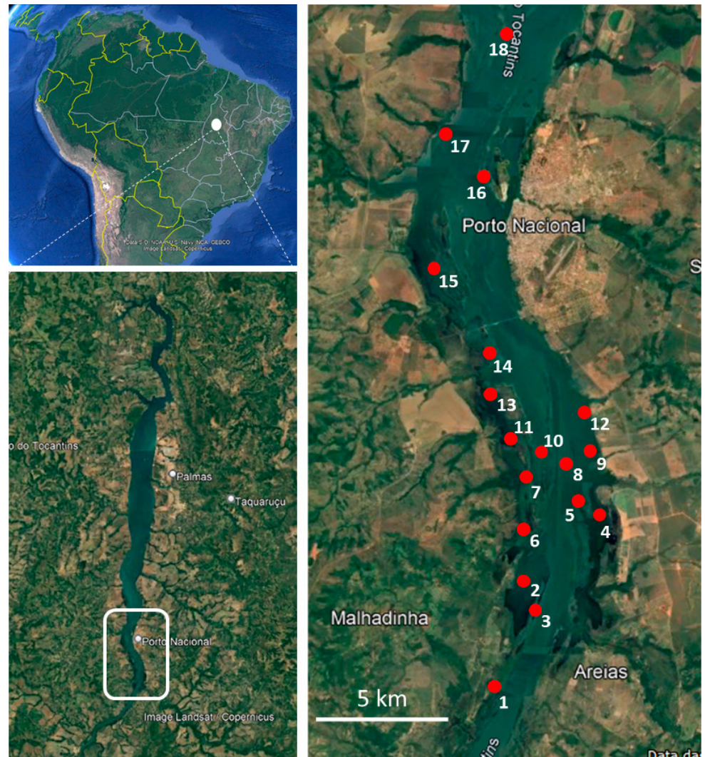
FIGURE S1 | Distribution of sampling sites ( n = 18 ) in the upper section of the Lajeado Reservoir, Tocantins River basin, Brazil. Satellite images were obtained from Google Earth Pro version 7.3.4.8573.
