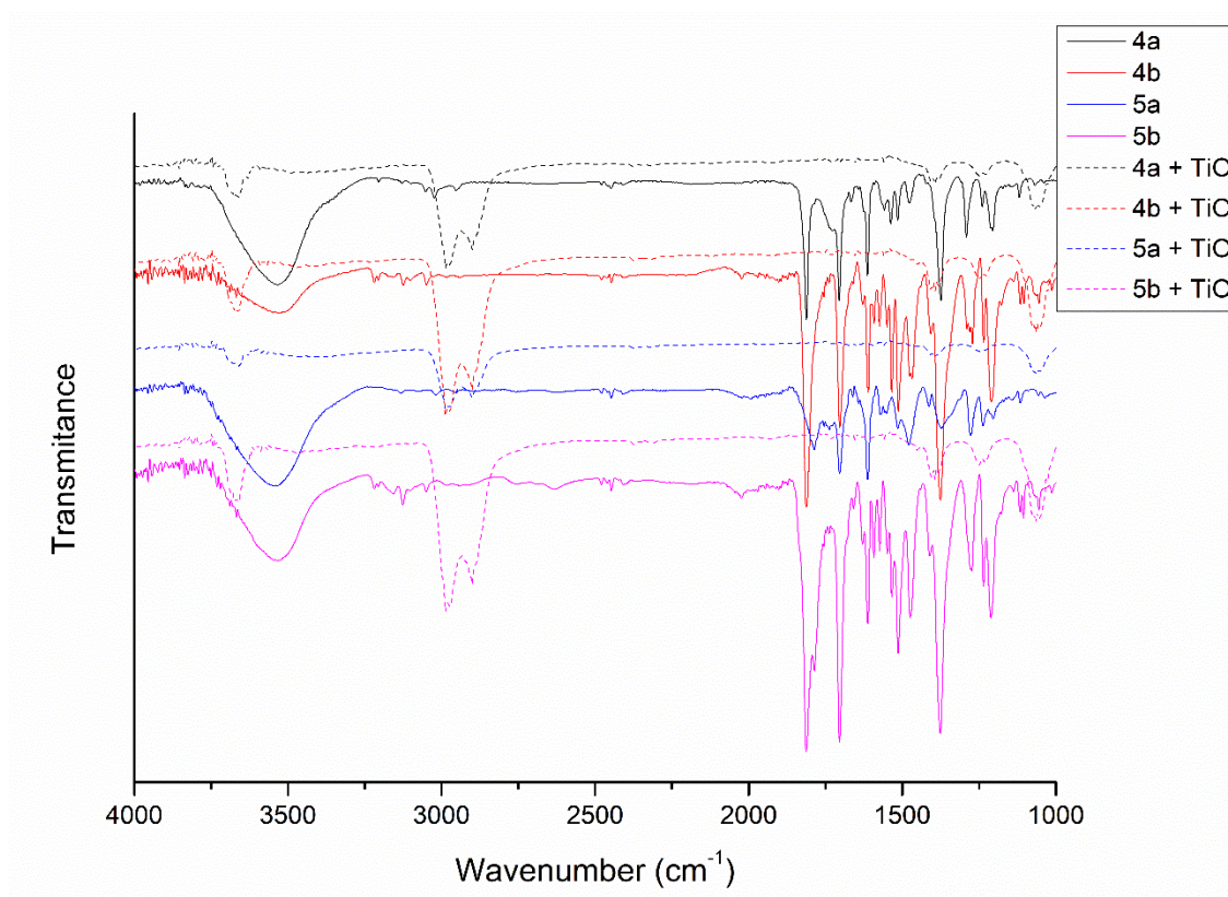
Figure S1 - FTIR comparison between free and TiO 2 -adsorbed dyes.
