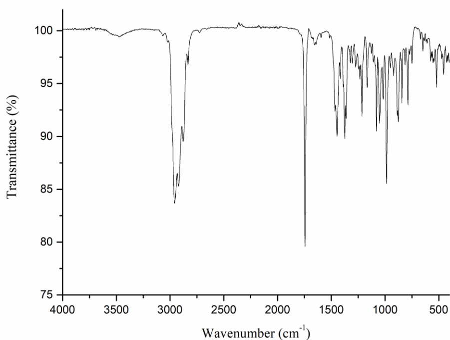
Figure S1 - Medium infrared spectra of rosemary essential oil (REO).
