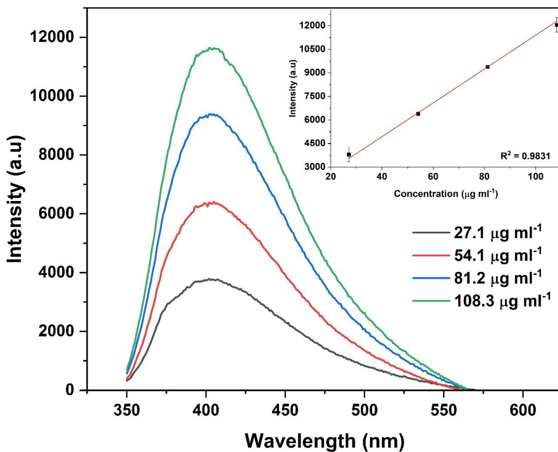
Figure S2 – Effect of variation in PQ-CDs concentration on emission intensity. Inset: linear correlation.
