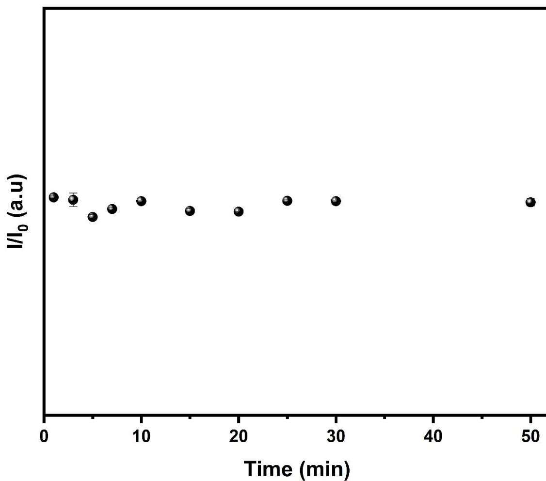
Figure S3 – Time effect on PQ-CDs fluorescence.
