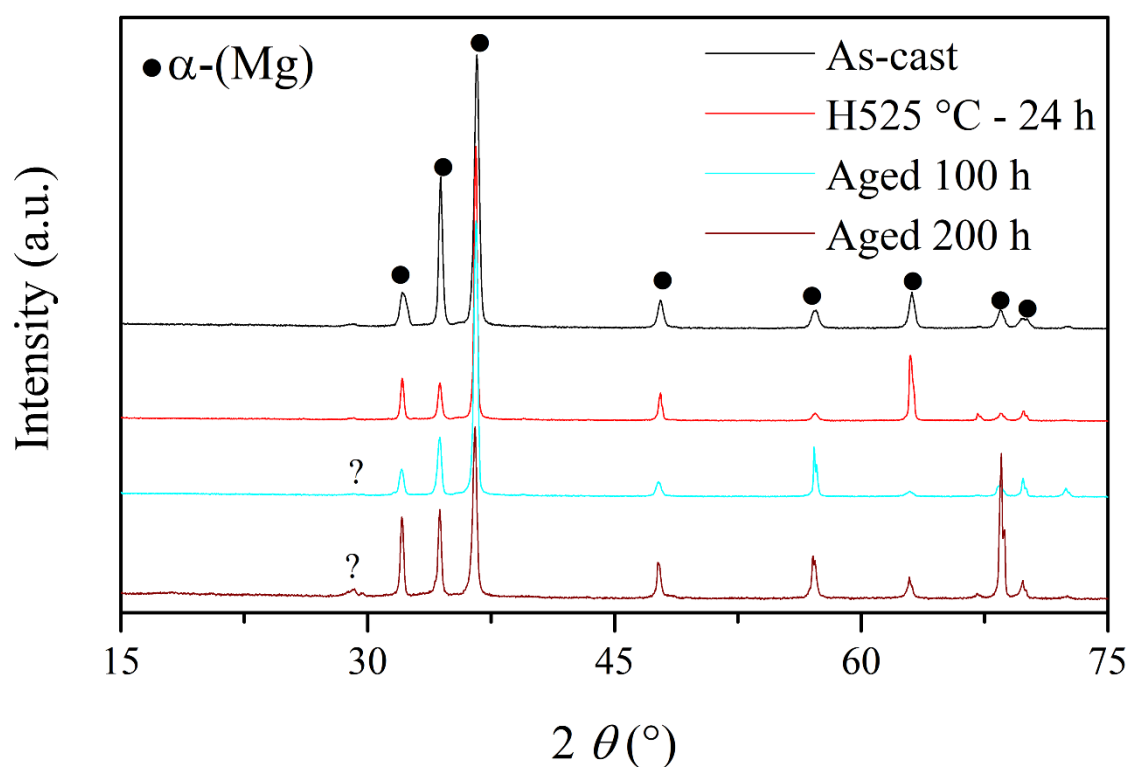
Figure S1 - XRD XRD patterns of the Mg–Y–Gd–Zr alloy in the as-cast, solution heat-treated (525 °C/24 h), and aged (100 h and 200 h) conditions.
