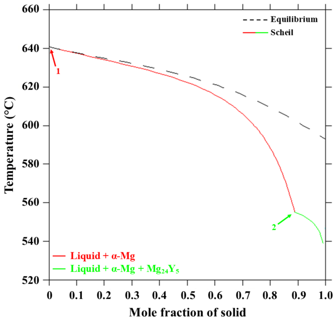
Figure S2 - Thermodynamic prediction of phase evolution during solidification of the Mg–Y–Gd–Zr alloy obtained by Thermo-Calc® using the Scheil–Gulliver approach.
