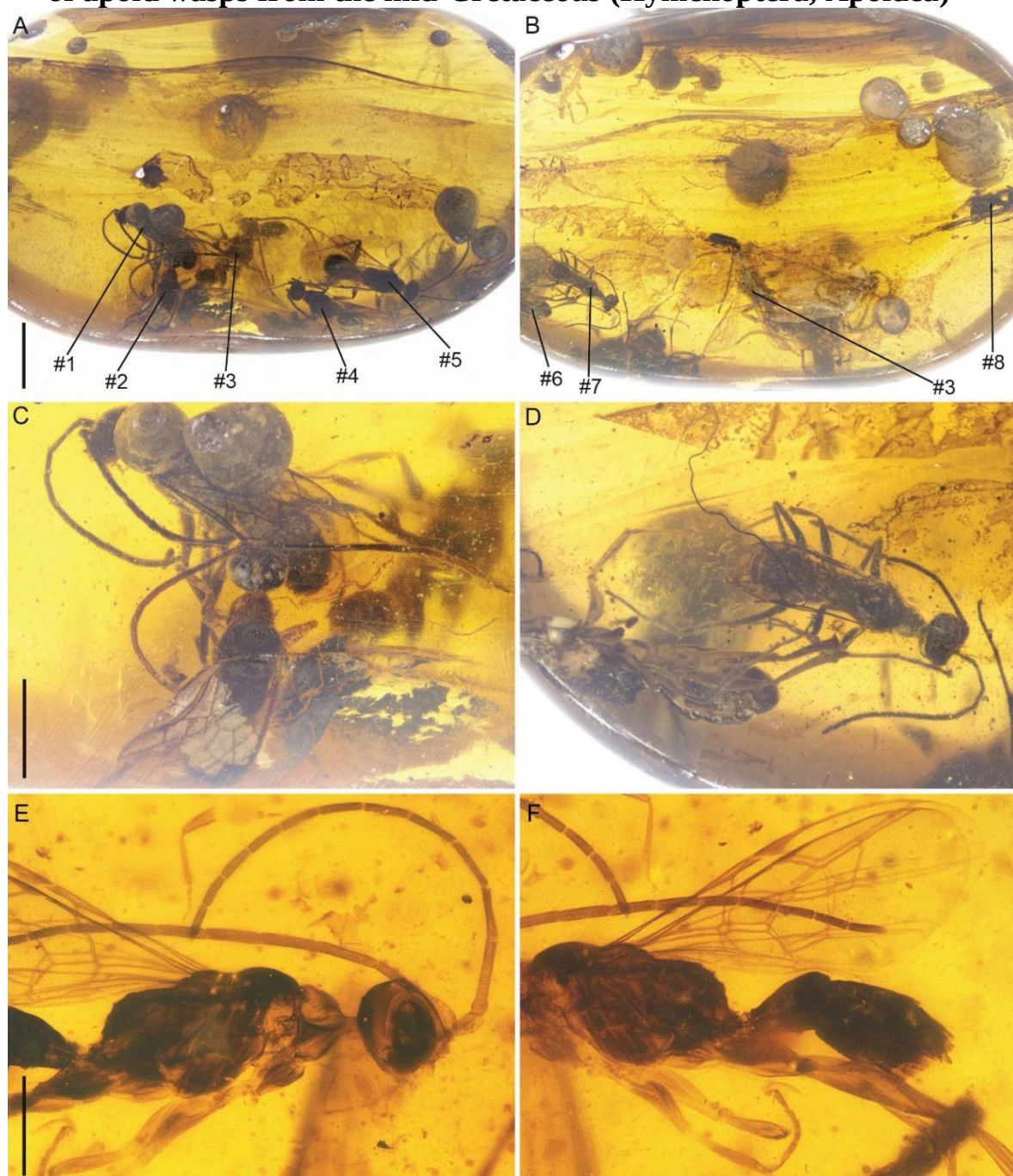
Figure S5 - Males of † Temnogyna multiplex sp. nov. (a, b) General view of the piece DZUP Bur-1559; (c) dorsal habitus of male #1 and #2; (d) dorsal habitus of male #7 and lateral view of male #6; (e) lateral of mesosoma and head of † Temnogyna multiplex sp. nov., male holotype (DZUP Bur-002a); (f) lateral of mesosoma and metasoma of † Temnogyna multiplex sp. nov., male holotype (DZUP Bur-002a). Scale bars, a, b: 2 mm; c, d: 1 mm; e, f: 0.5 mm.
