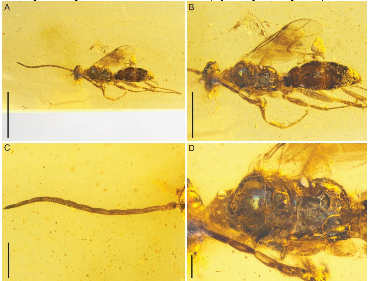
Figure S3 - Male of † Temnogyna aff. elegans sp. nov. (DZUP Bur-208). (a) Dorsal habitus; (b) dorsal habitus; (c) general view of antenna; (d) dorsal view of mesosoma. Scale bars, a : 2 mm; b : 1 mm c : 0.5 mm; d : 0.2 mm.
