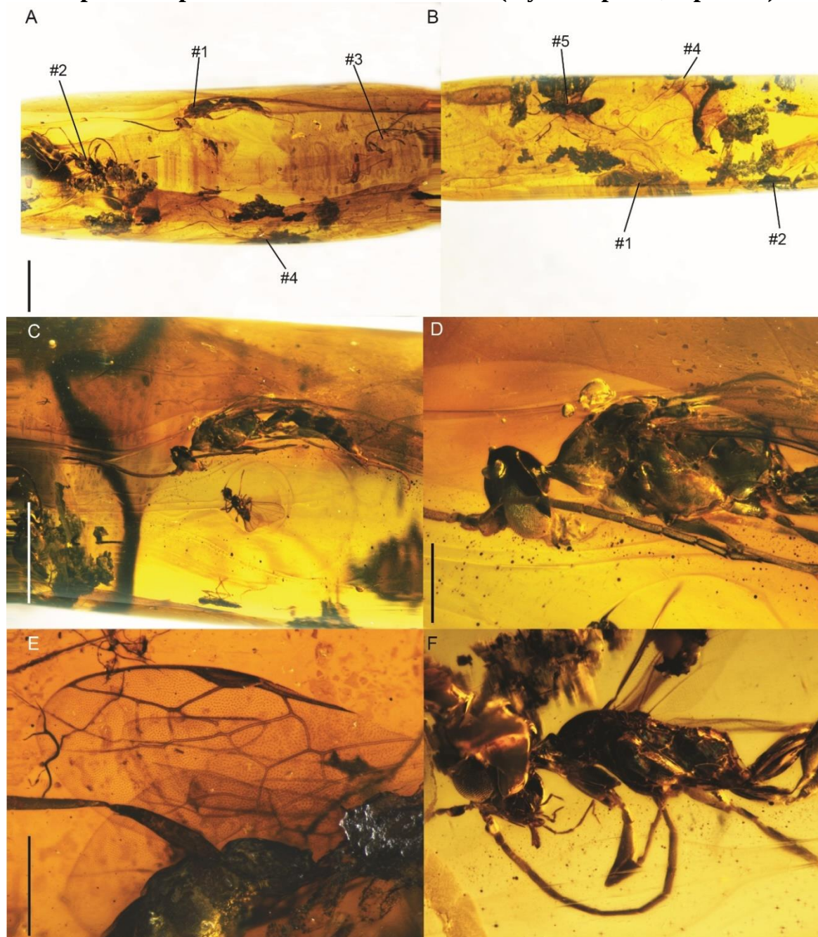
Figure S2 - Males of † Temnogyna aff. elegans sp. nov. (DZUP Bur-534). (a, b) General view of the piece DZUP Bur-534; (c) lateral habitus of male #1; (d) lateral view of head and mesosoma of male #1; (e) anterior and posterior view wings of male #5; (f) ventral view of head and lateral view of mesosoma of male #2. Scale bars, a, b : 2 mm; c, d : 0.5 mm; e : 0.5 mm.
