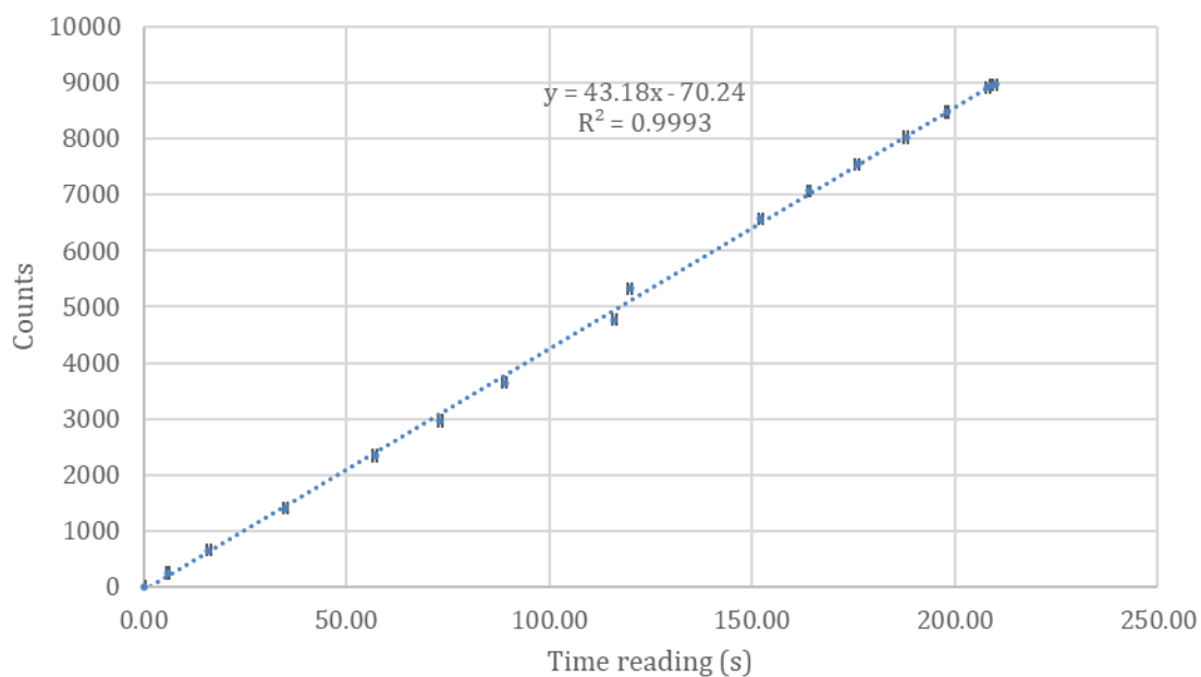
Figure S2: Accumulated counts as a function of measurement time during irradiation with a certified Cs-137 reference source at a secondary standard dosimetry laboratory.
