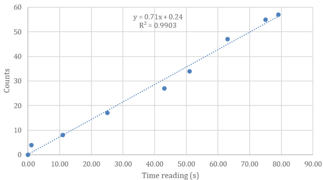
Figure S1: Accumulated counts as a function of measurement time for environmental background radiation.
