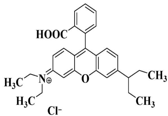
Figure 1S. Chemical structure of the Rhodamine B in this work
