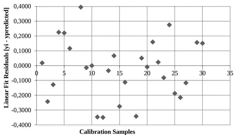
Figure S1. Dispersion of residues from the analytical curve obtained from the application of GC-MS.
