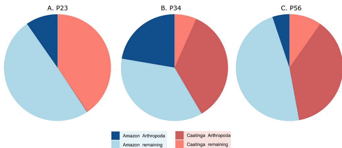
Figure S4 - Pie charts representing the proportion of reads recovered by biome (Amazon blue, Caatinga red) and the proportion of Arthropoda reads by biome for each primer pair dataset.
