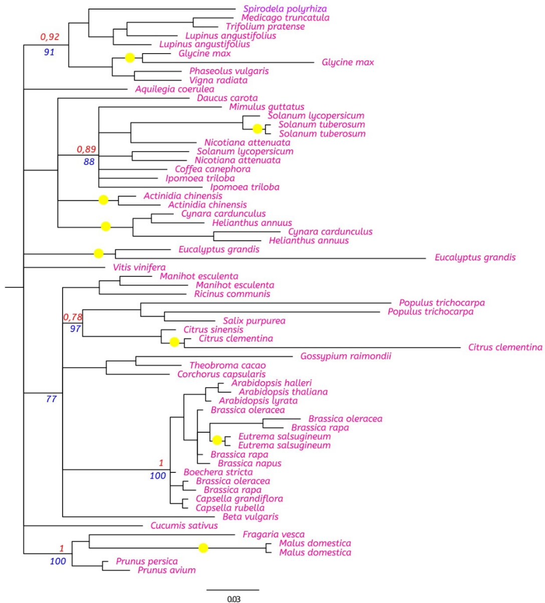
Figure S5 - Phylogenetic relationships among PSY genes belonging to Subgroup E2 from Figure 1 presents both posterior probability (numbers in red) with a cut-off point of 0,8 and bootstrap values (numbers in blue) with a cut-off point of 70. Yellow circle represents the duplication events. The complete list of species is presented in Table S1.
