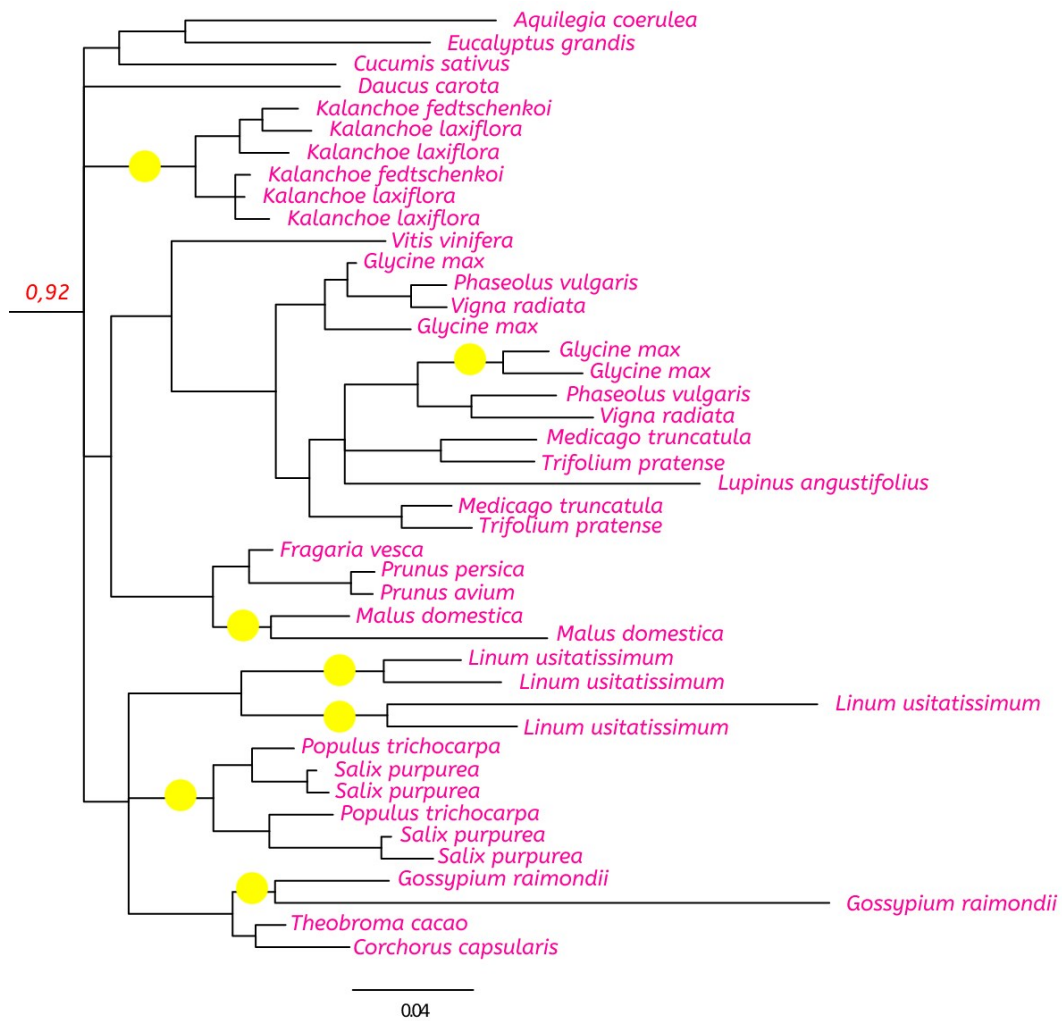
Figure S4 - Phylogenetic relationships among PSY genes belonging to Subgroup E1 from Figure 1 presents both posterior probability (numbers in red) with a cut-off point of 0,8 and bootstrap values (numbers in blue) with a cut-off point of 70. Yellow circle represents the duplication events. The complete list of species is presented in Table S1.
