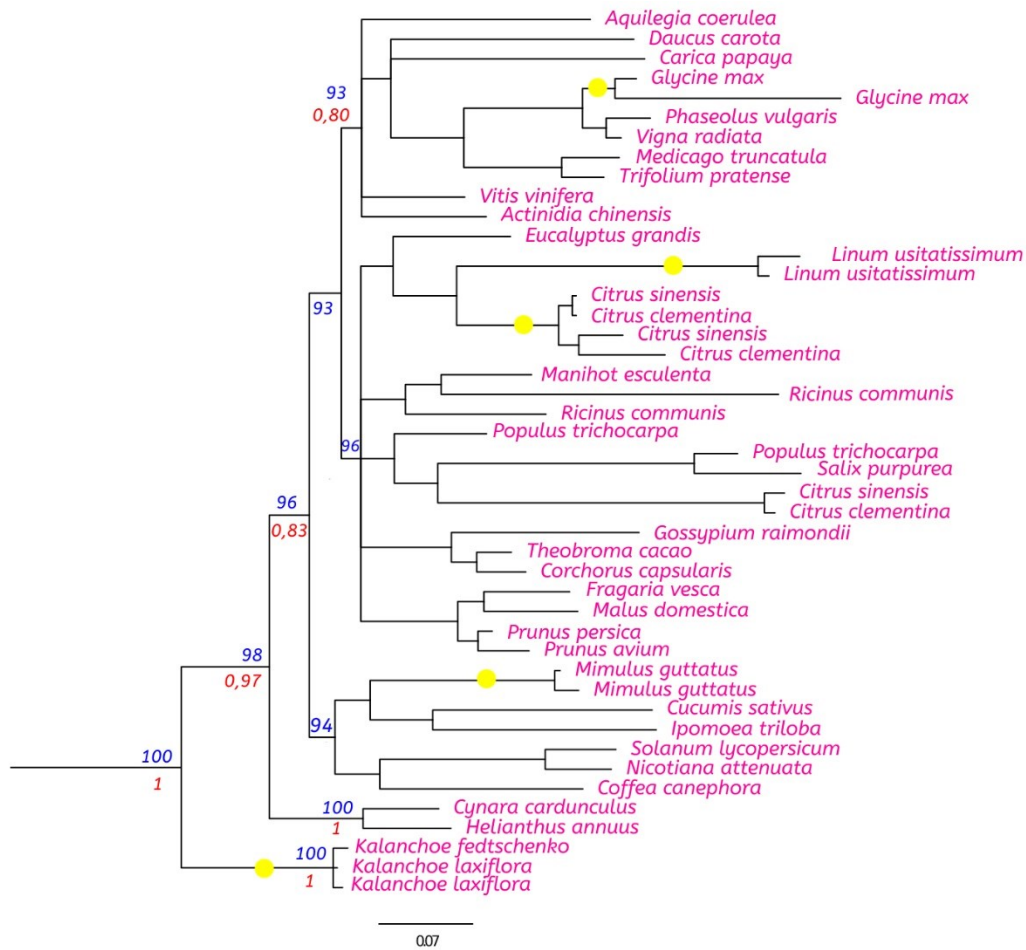
Figure S3 - Phylogenetic relationships among PSY genes belonging to subgroup E3 from Figure 1 presents both posterior probability (numbers in red) with a cut-off point of 0,8 and bootstrap values (numbers in blue) with a cut-off point of 70. Yellow circle represents the duplication events. The complete list of species is presented in Table S1.
