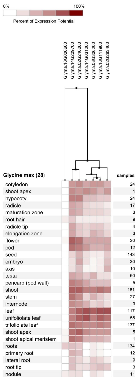
Figure S10 - Gene expression analysis across anatomical parts of G. max performed using GENEVESTIGATOR.
