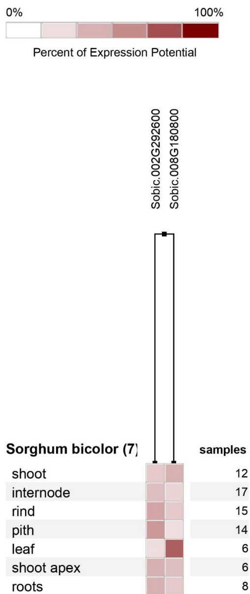
Figure S15 - Gene expression analysis across anatomical parts of S. bicolor performed using GENEVESTIGATOR.
