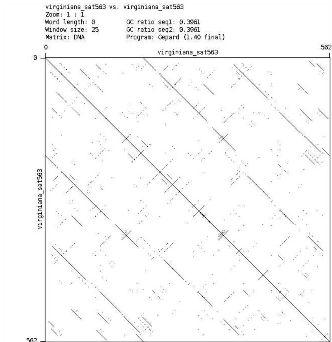
Figure S7 - Self-similarity dot-plot of sat563 demonstrating it may be composed of smaller segments of repetitive DNA.
