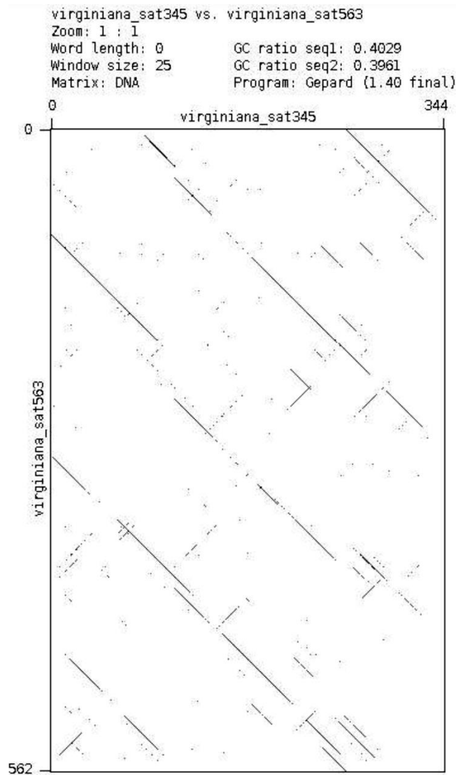
Figure S3 - Dot-plot demonstrating that sat345 is embedded within sat563.
