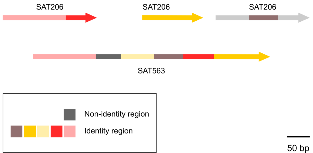
Figure S9 - Schematic diagram depicting the identity relationship between SAT206 and SAT563.
