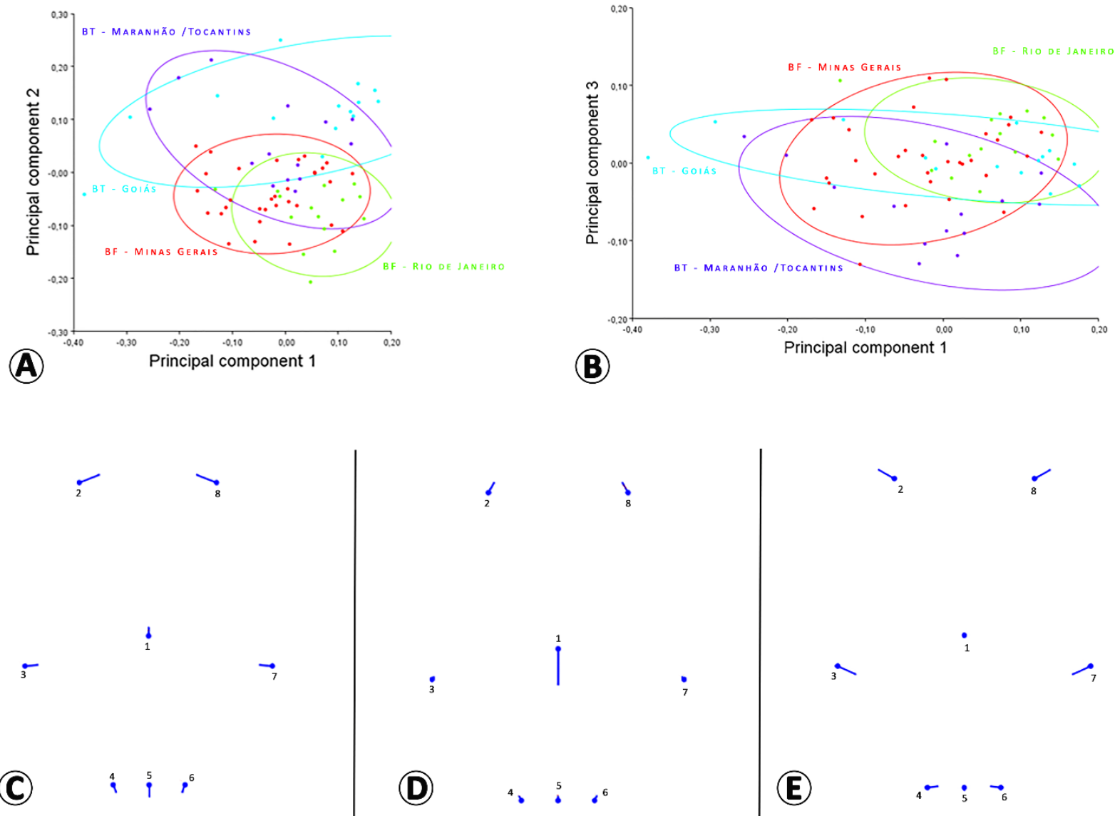
Figure S3. Principal Component Analysis (PCA) of morphometrics of populations of B. fusconervis (BF) and B. tenella (BT). A. PC1+PC2 axis. B. PC1+PC3 axis. C. Variation observed in PC1. D. Variation observed in PC2. E. Variation observed in PC3.
