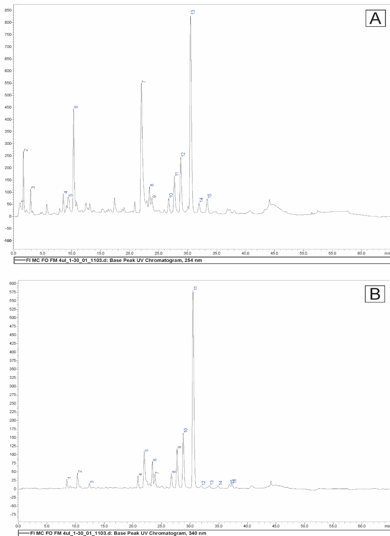
Figure S5: Chromatograms obtained for the methanolic fraction of Miconia cinnamomifolia (DC) Naudin. from the Dense Ombrophilous Forest at 254 nm (A) and 340 nm (B).
