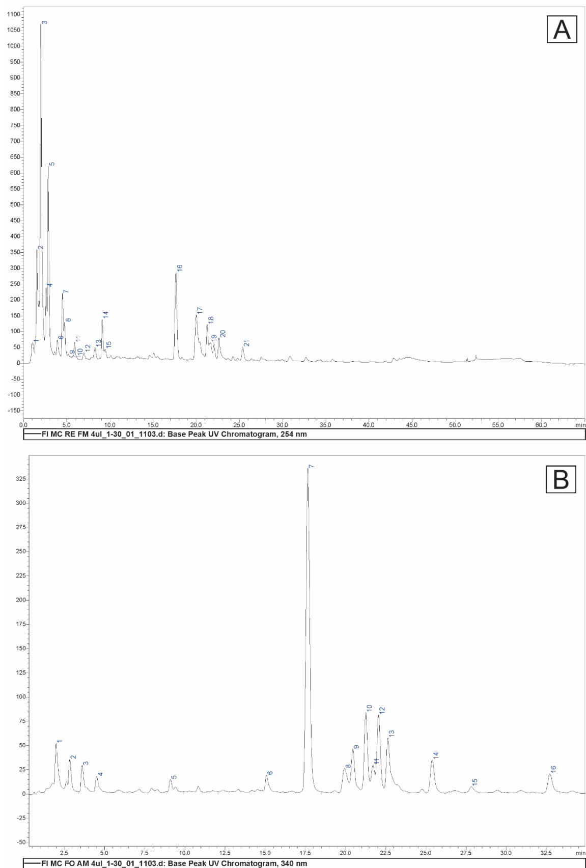
Figure S6: Chromatograms obtained for the methanolic fraction of Miconia cinnamomifolia (DC) Naudin. from the Restinga at 254 nm (A) and 340 nm (B).
