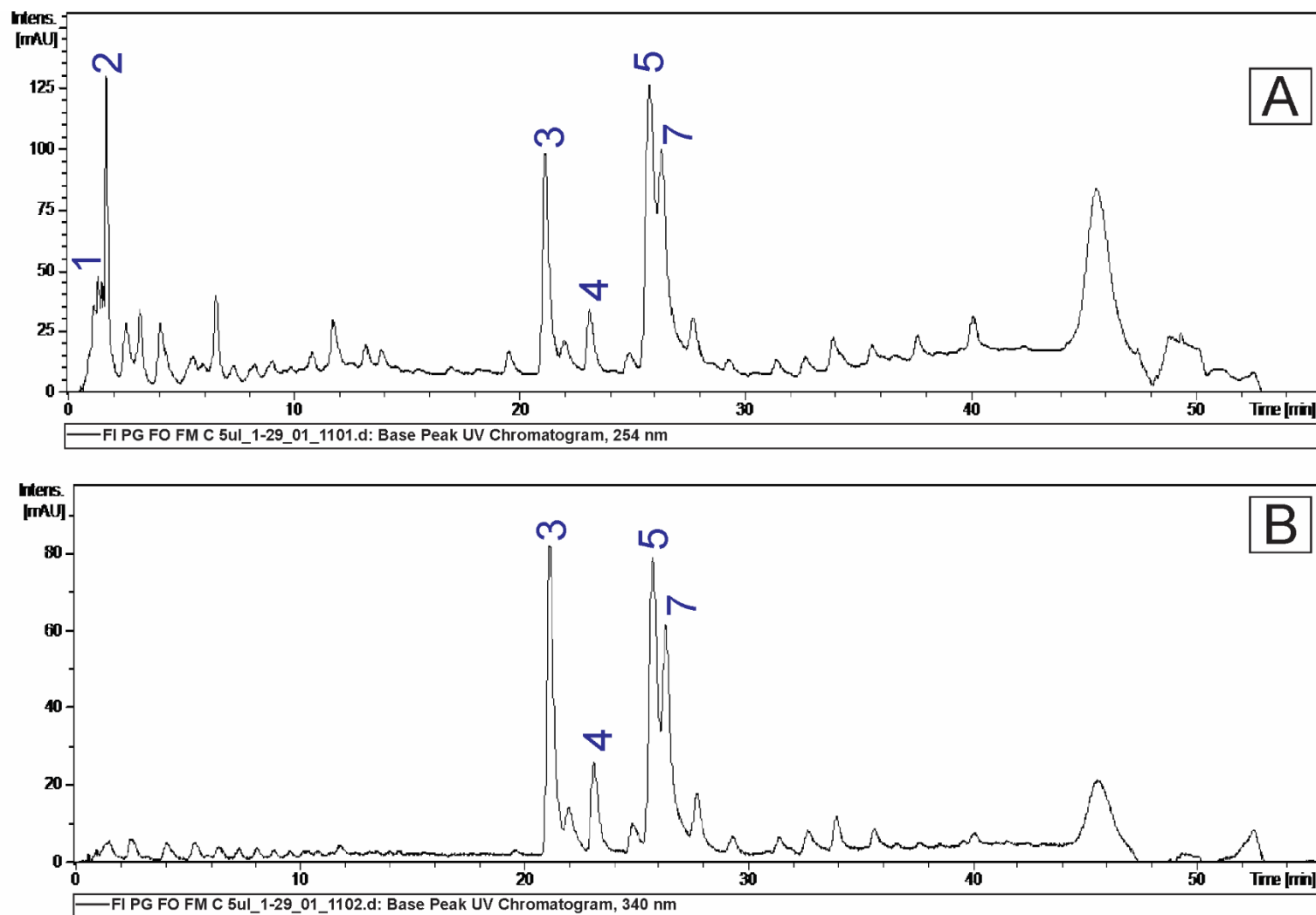
Figure S3: Chromatograms obtained for the methanolic fraction of Psidium guineense Sw. from the Dense Ombrophilous Forest at 254 nm (A) and 340 nm (B).
