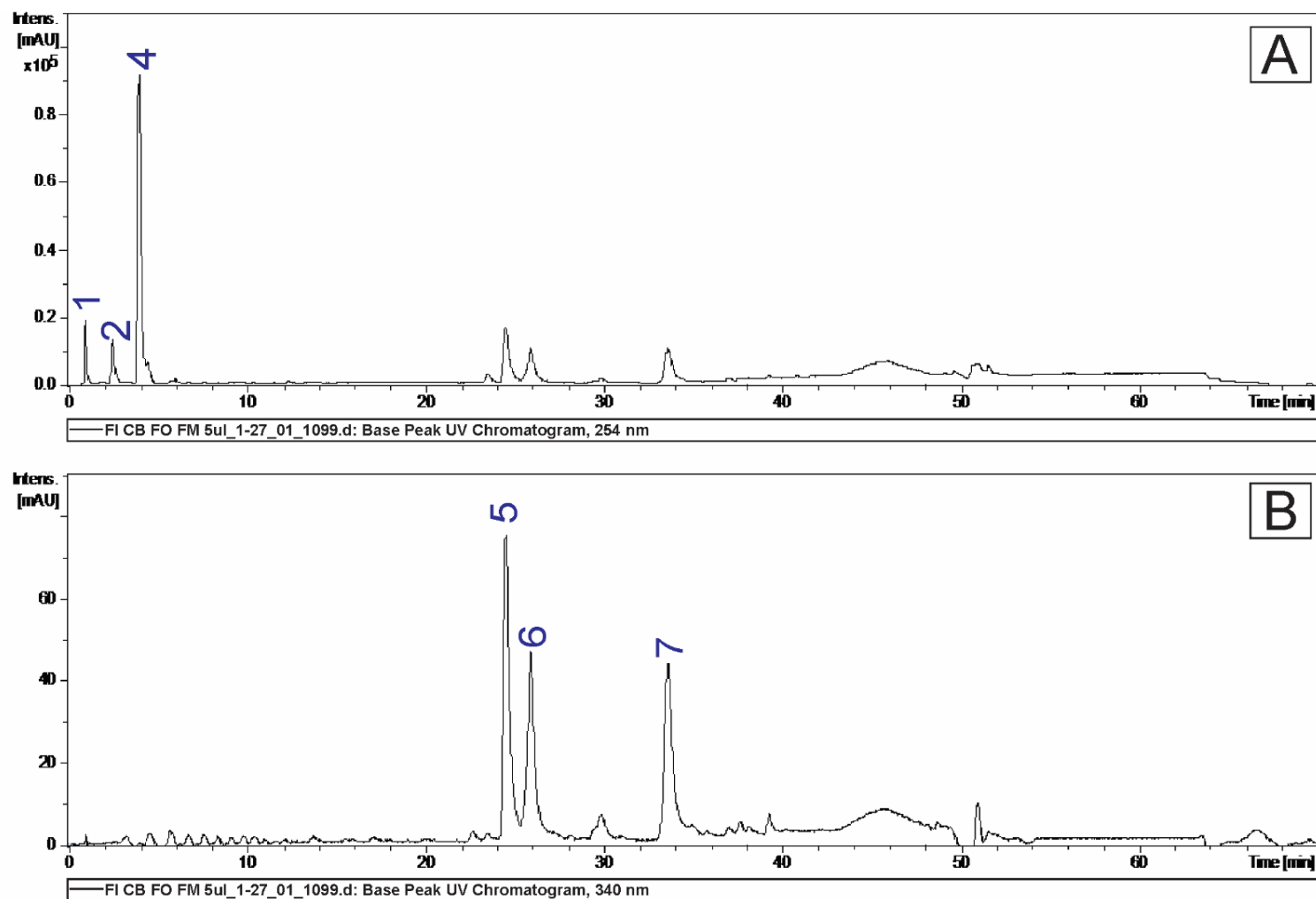
Figure S1: Chromatograms obtained for the methanolic fraction of Calophyllum brasiliense from the Dense Ombrophilous Forest at 254 nm (A) and 340 nm (B).
