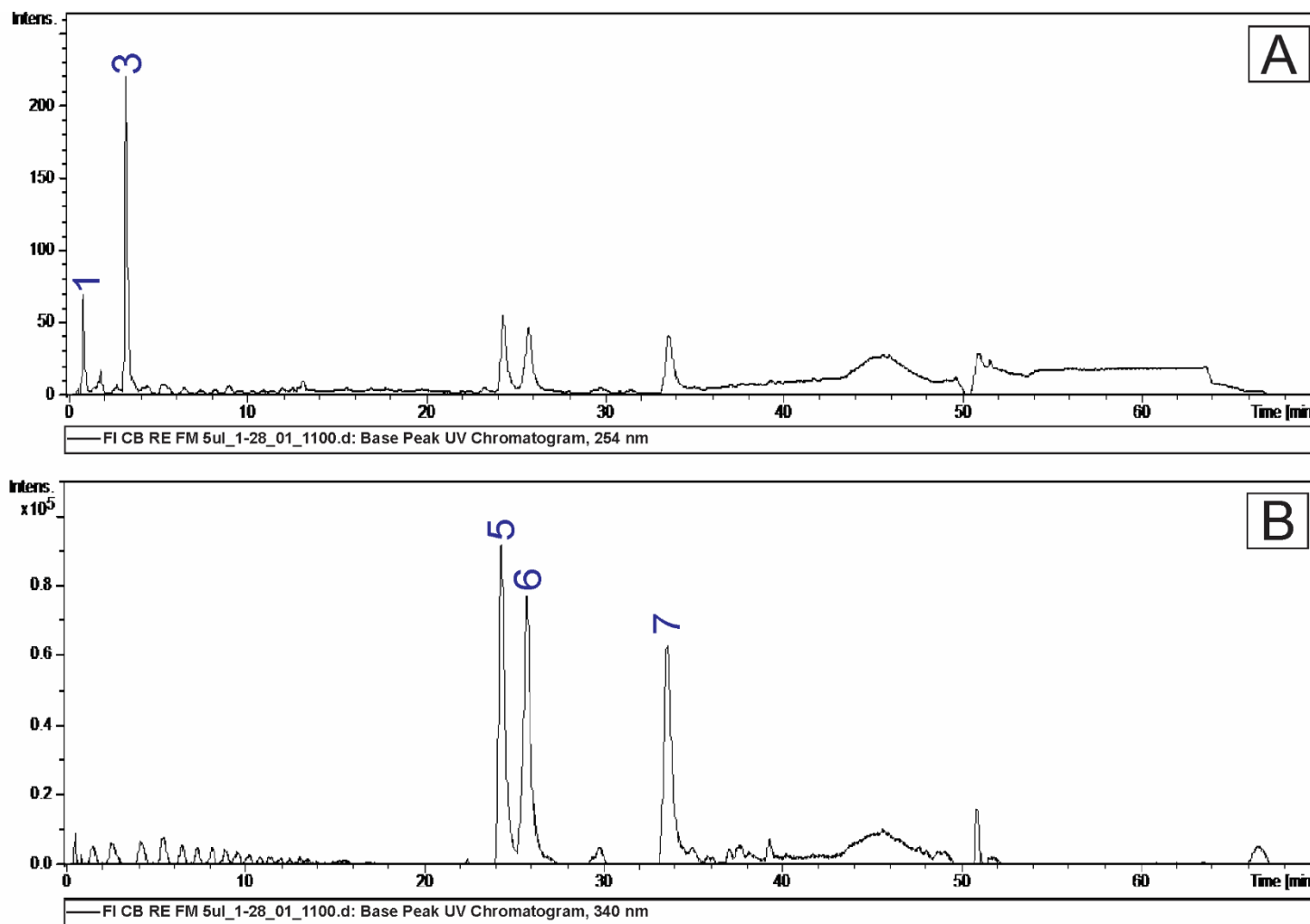
Figure S2: Chromatograms obtained for the methanolic fraction of Calophyllum brasiliense from the Restinga at 254 nm (A) and 340 nm (B).
