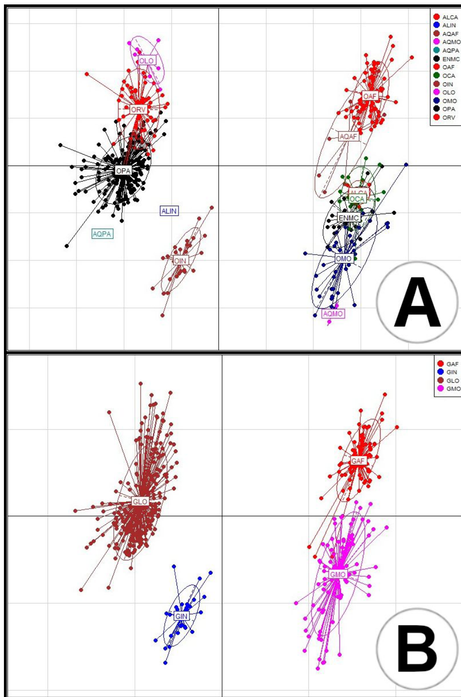
Figure S1. A – PCoA for thirteen morphological types previously identified using the adapted identification key, where the variable LOC is unweighted. B – PCoA for the groups, labeled according to the four cohesive groups identified and discussed in the text.
