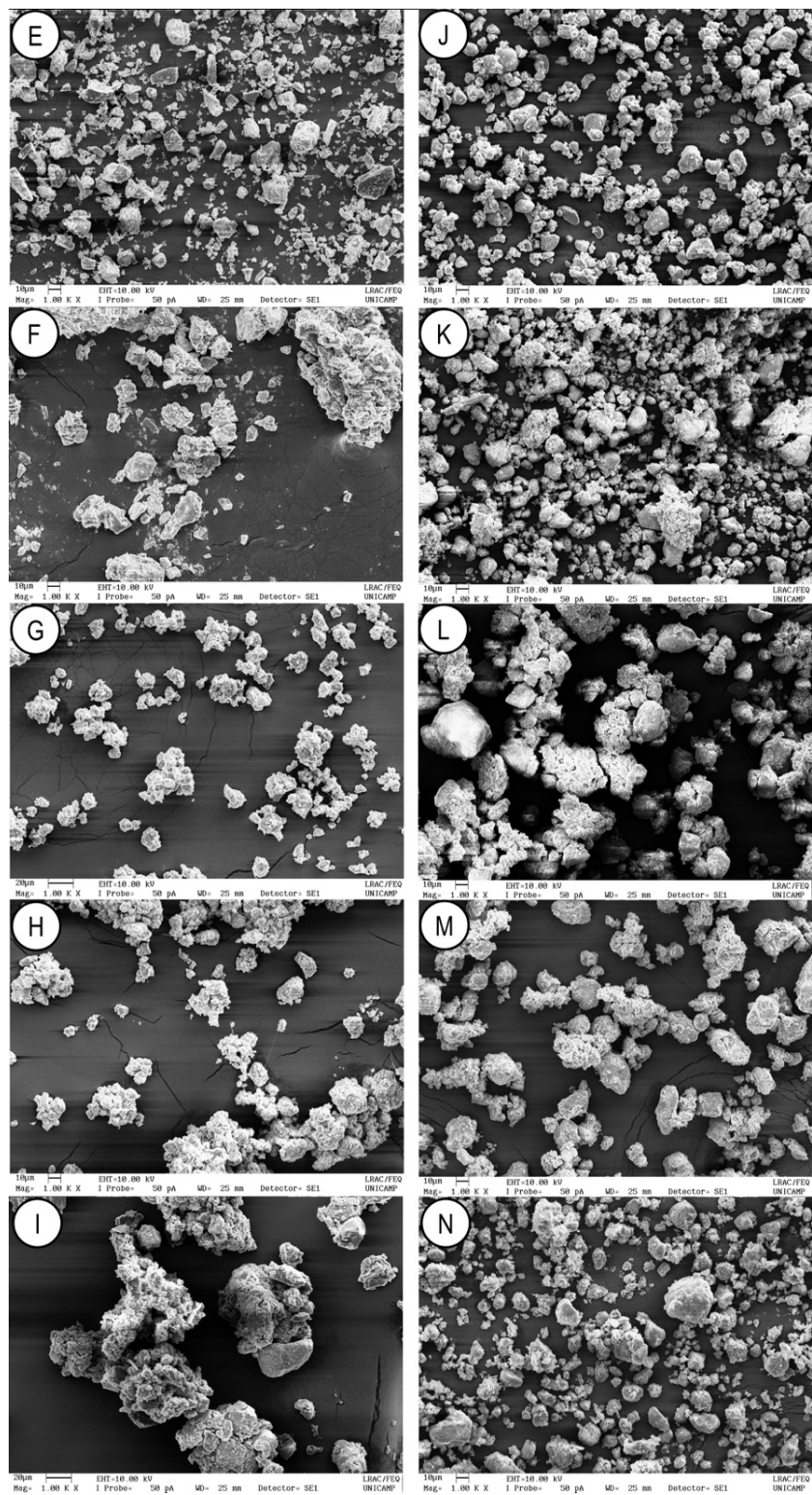
Supplementary Figure 4. Images of whitening toothpastes by SEM (1000×). The codes are presented in the table of supplementary material.
