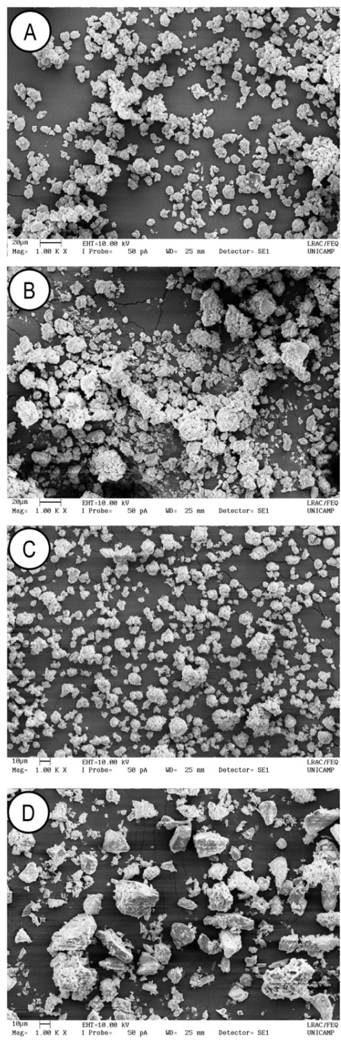
Supplementary Figure 3. Images of regular toothpastes by SEM (1000×). The codes are presented in the table of supplementary material.
