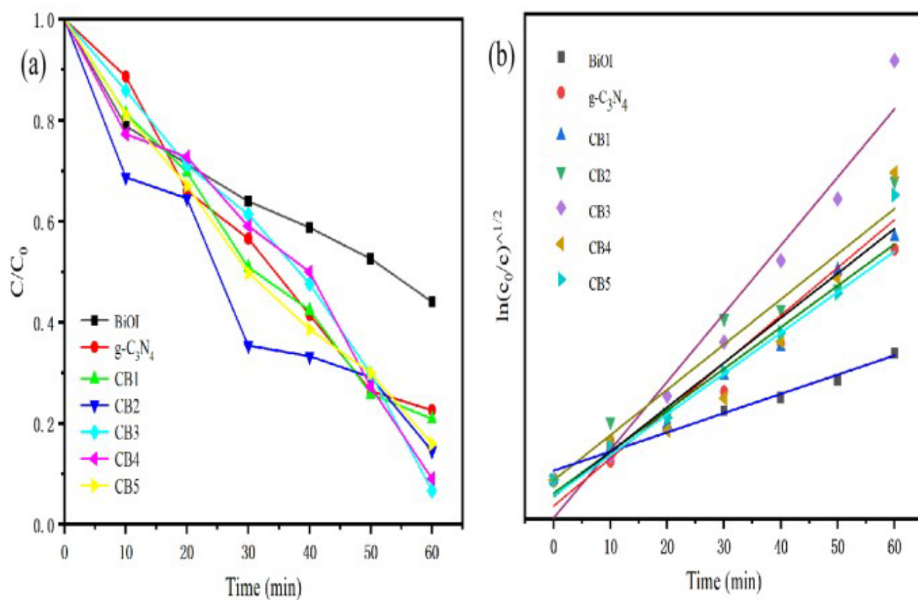
Figure S5 - Photocatalytic degradation of precursor g-C 3 N 4 BiOI in RhB solution (20 mg/L) under visible light irradiation(a), first-order kinetic fitting curve (b).
