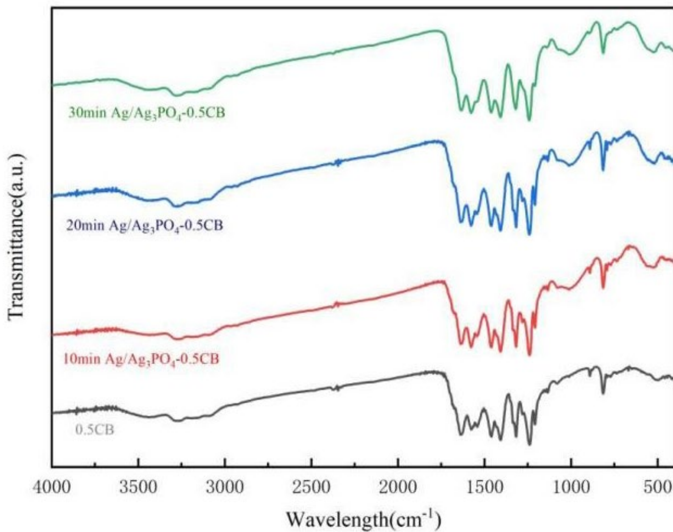
Figure S8 - FT-IR pattern of Ag/Ag 3 PO 4 -CB3 photocatalyst.
