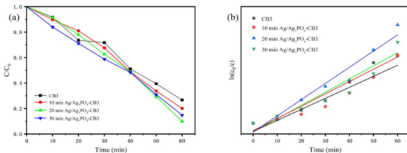
Figure S13 - Photocatalytic degradation of Ag/Ag 3 PO 4 -CB3 photocatalyst in CIP solution (10mg/L) under visible light irradiation (a), first-order kinetic fitting curve (b).
